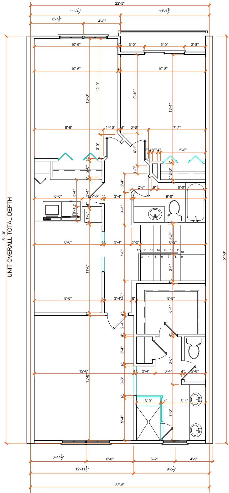
CENTER UNIT - SECOND FLOOR
