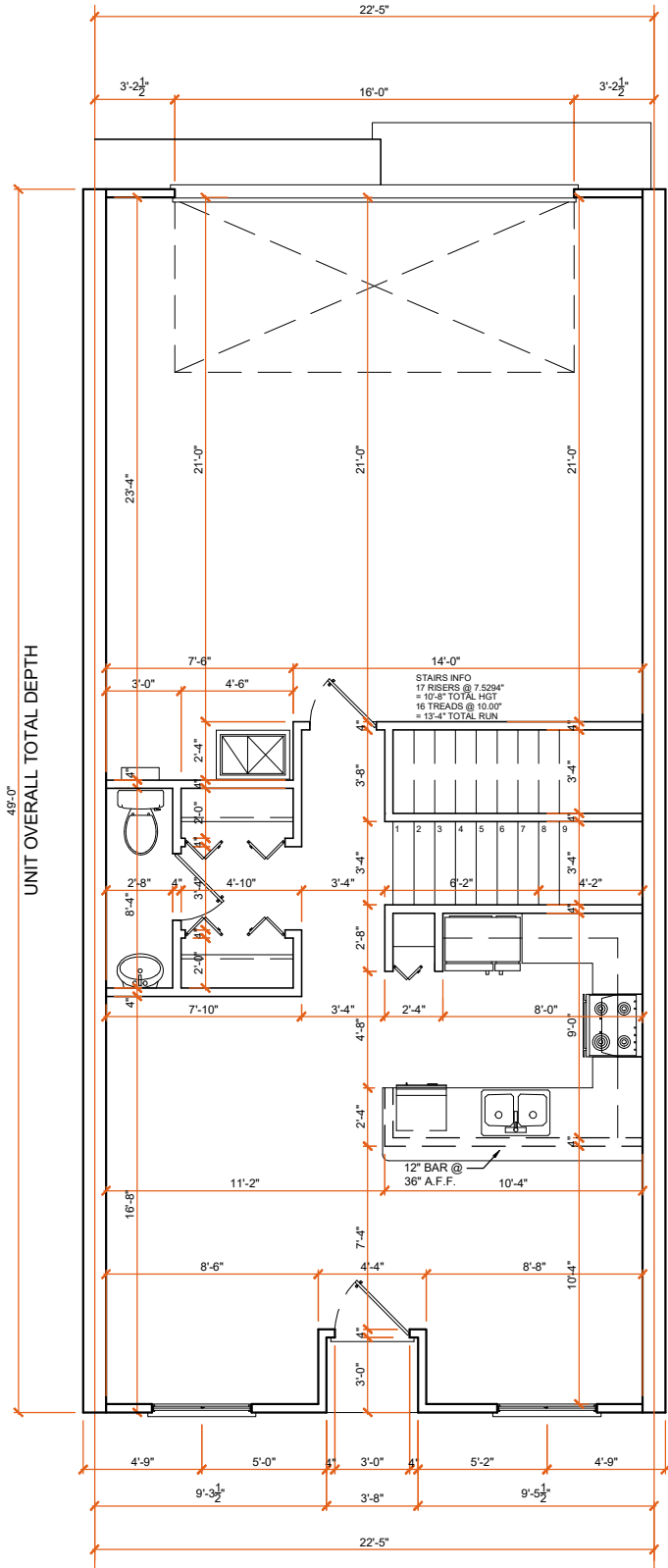
CENTER UNIT - FIRST FLOOR
